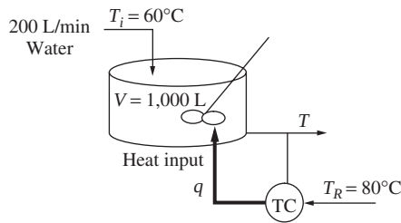
FIGURE 12-3 Stirred-tank heater control system.
