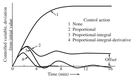
(Figure 9.10 Response of a typical control system showing the effects of various modes of control.)
