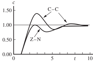
FIGURE 18–12 Response to unit-step change in set point for the system in Fig. 18–11 (Example 18.3).
