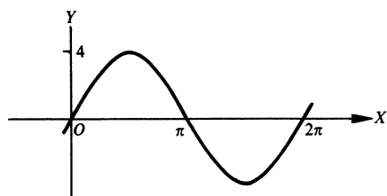
(a) y = 4 \sin x
