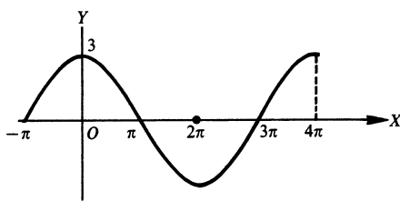
(e) y = 3 \cos \frac{1}{2}x
