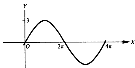
(c) y = 3 \sin \frac{1}{2}x
