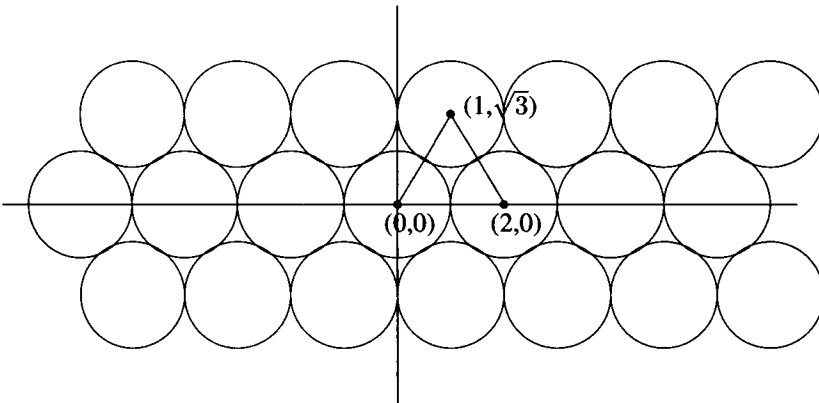
Figure 6.7 A lattice packing with contact number 6 and density \doteq 0.90 .
