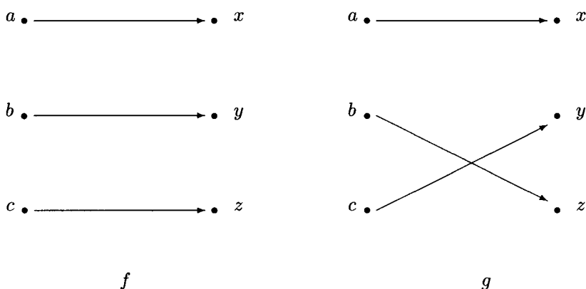
Figure 2.4 Two functions. Are they equivalent?
