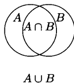
Figure 1.3 A Venn diagram for two sets.
