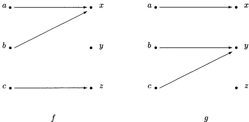
Figure 2.5 Equivalent functions when domain and codomain are unlabeled.
