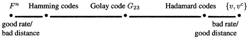
Figure 6.5 The world of codes.
