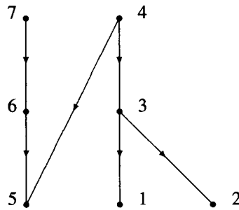
Figure 3.3 A partial order of width 3 and length 3.
