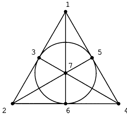
Figure 5.2 The Fano Configuration (FC).
