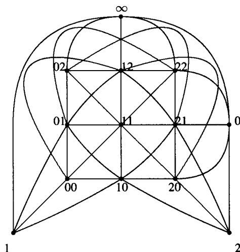
Figure 6.1 A projective plane of order 3.
