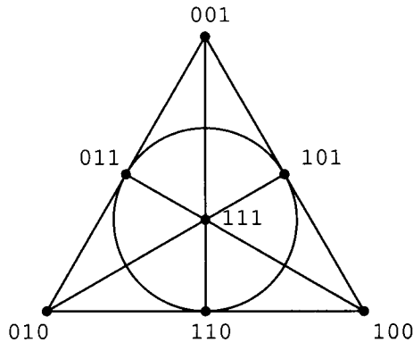
Figure 5.3 A vector representation of FC.
