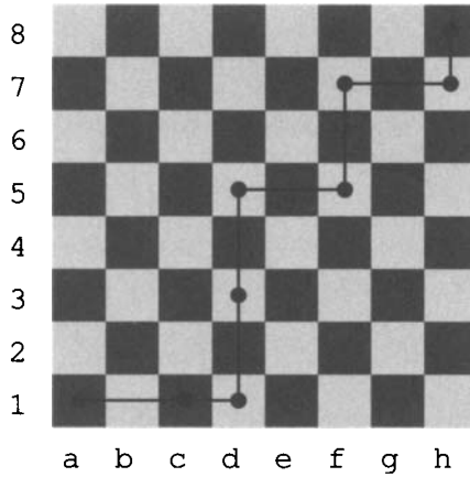
Figure 2.1 A Rook walk from a1 to h8.
