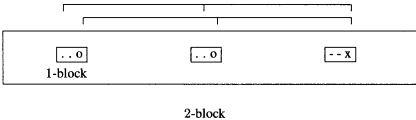
Figure 4.3 Two 3-APs focusing on an integer.
