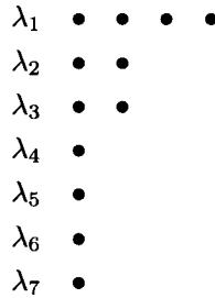
Figure 2.3 A transpose Ferrers diagram.
