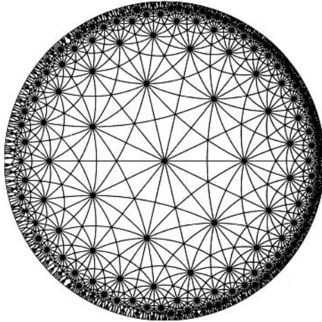
Figure 5.4 A triangle tiling of the hyperbolic plane.
