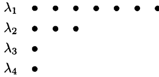
Figure 2.2 The Ferrers diagram of a partition of 12.
