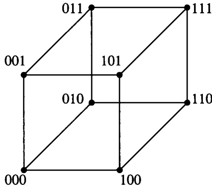
Figure 5.1 F^3 as the set of vertices of a cube.
