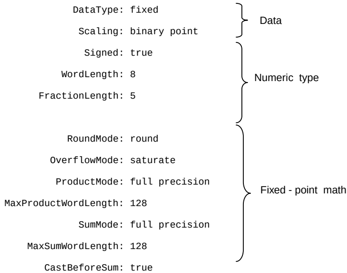
Figure 3.20 MATLAB® support for fixed point arithmetic
