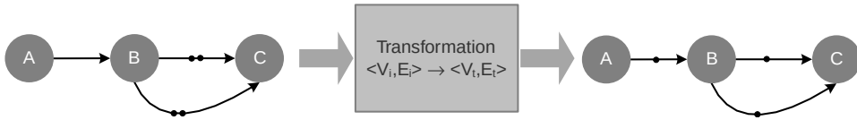
Figure 4.30 Mathematical transformation changing a DFG to meet design goals
