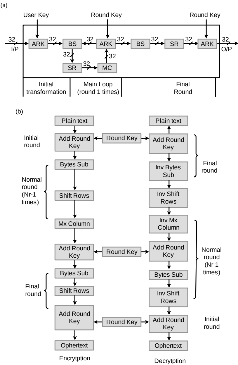
Figure 13.24 AES algorithm. (a) Block diagram of encryption. (b) Flow of algorithm for encryption and decryption
