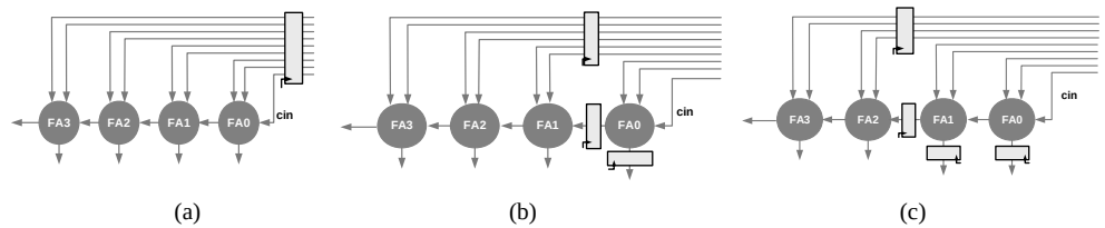
Figure 7.10 Node transfer theorem to add one level of pipeline registers in a 4 bit RCA. (a) the original DFG. (b) Node transfer theorem applied around node FA0. (c) Node transfer theorem applied around FA1
