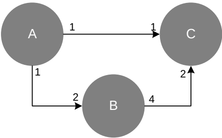
Figure 4.42 SDFG for computing a non trivial solution (exercise 4.6)
