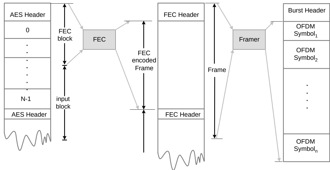
Figure 13.40 Header and frame insertion for synchronization
