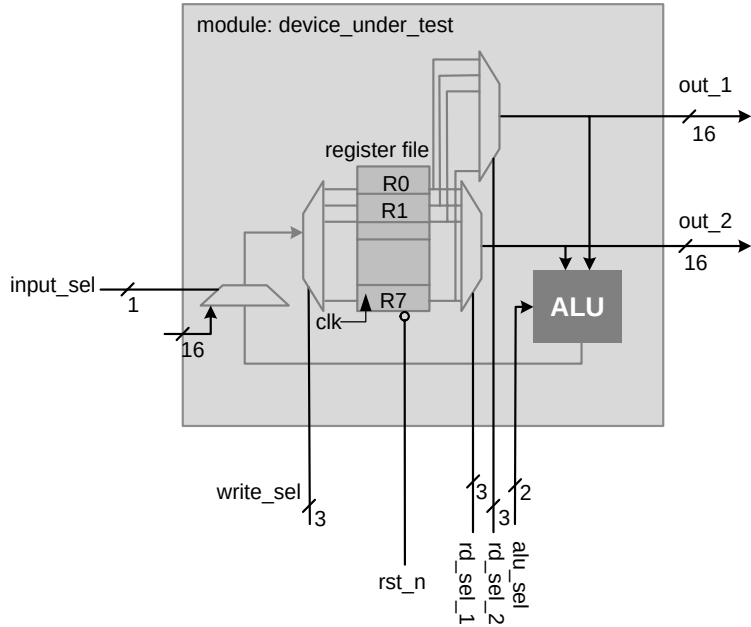
Figure 2.23 Digital design with multiple inputs and outputs
