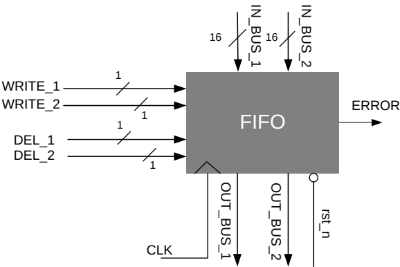
Figure 10.27 FIFO top level design for exercise 10.3
