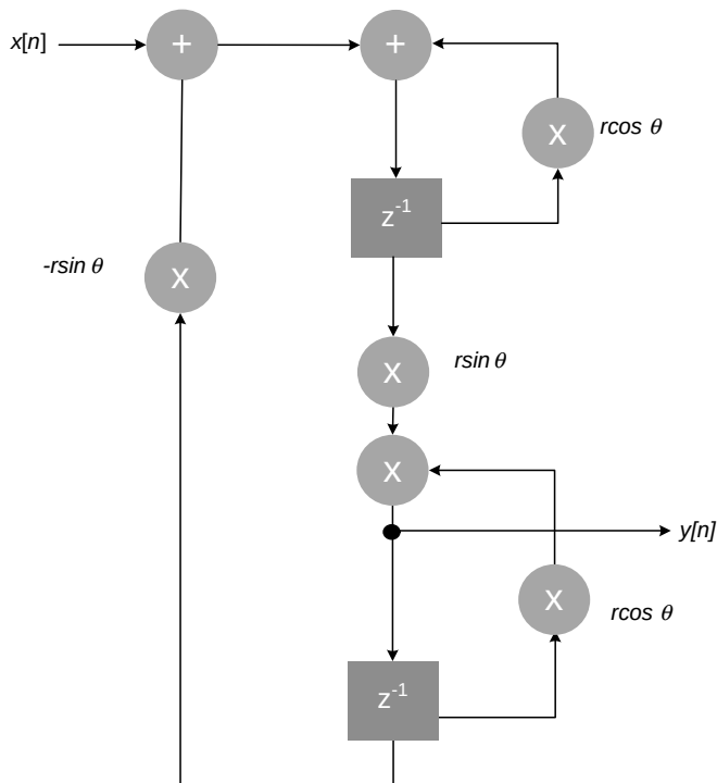
Figure 3.30 Filter structure to place quantized pole pair \text{re}^{\pm j\theta} at intersections of evenly placed horizontal and vertical lines inside the unit circle
