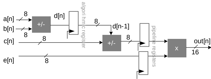
Figure 4.35 Pipelining while maintaining coherency in the datapath
