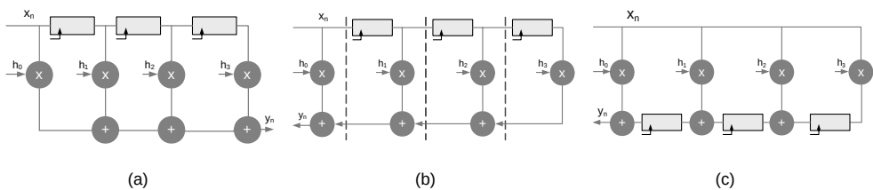
Figure 7.6 FIR filter in direct form transformation to a TDF structure using cut set retiming. (a) A 4 coefficient FIR filter in DF. (b) Reversing the direction of additions in the DF and applying cut set retiming. (c) The retimed filter in TDF
