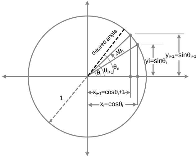
Figure 12.6 CORDIC algorithm incremental rotation by \Delta\theta_i
