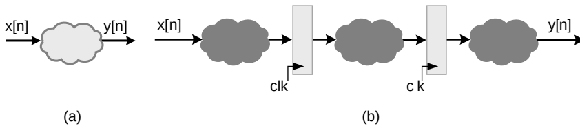
Figure 7.1 Pipeline registers are added to reduce the critical path delay of a combinational cloud. (a) Original combinational logic. (b) Design with three levels of pipelining stages with two sets of pipeline registers
