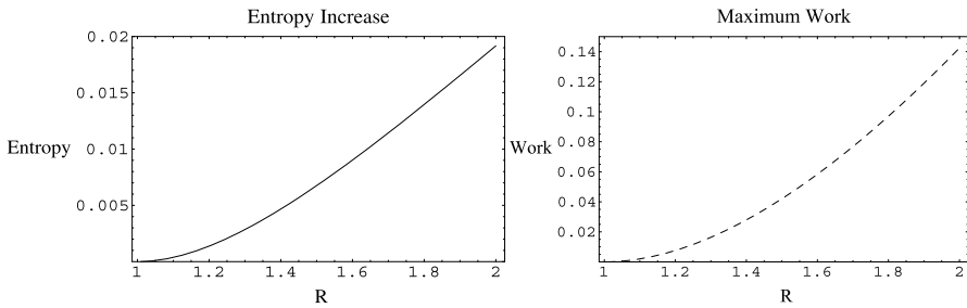
Fig. 4.8 (a) Setting C\rho AL = 1 and T_1 = 1 , the entropy difference, S_{\text{eq}} - S_0 , is plotted as a function of the temperature ratio R = T_2/T_1 . (b) With C\rho AL set equal to 1, the total work extracted, W_{\text{max}} , is plotted as a function of the temperature ratio R = T_2/T_1 . For simplicity, T_1 is again set equal to 1
