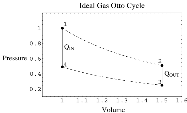
Fig. 4.11 Otto cycle using ideal gas as the working substance
