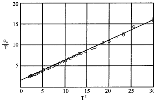
Fig. 11.18 \frac{c_v}{T} for sodium versus T^2 . Following the work of [28], the specific heat, C_v , of Na divided by the temperature, T , is plotted as a function of T^2 . Notice that the plot has an intercept at T \rightarrow 0 indicating that at very low temperature C_v has a linear dependence on T . For slightly higher temperature, the specific heat is seen to follow the T^3 law which is a result of the lattice vibrations. (See Fig. 11.19 and the related text for details of the lattice contribution)
