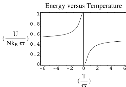
Fig. 11.14 Energy U , in units of Nk_B w , as a function of temperature T , in units of w , for a two state nuclear paramagnet. Notice that the energy is equal to zero—which is its minimum value—at T = +0 . It rises with the increase in temperature and levels off at \frac{Nk_B w}{2} as the temperature heads upward in the direction of T \rightarrow +\infty . Just beyond T = +\infty is T = -\infty . (Note, in theory, all negative temperatures are higher than +\infty .) From here, as the temperature moves “upwards” toward T = -0 , the energy slowly rises above \frac{Nk_B w}{2} and reaches its maximum value of Nk_B w at the end of its journey at T = -0
