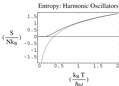
Fig. 11.6 Entropy of a quantum and a classical simple harmonic oscillator. The solid curve represents the entropy of a quantum simple harmonic oscillator as a function of the dimensionless variable \gamma^{-1} = \frac{k_B T}{\hbar\omega} . The entropy is given in units of k_B . The dashed curve represents the corresponding result for a classical simple harmonic oscillator
