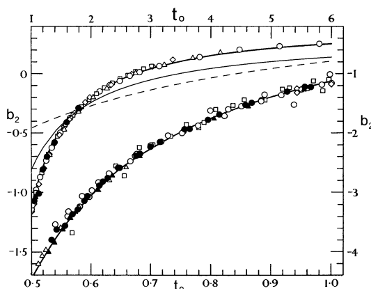
Fig. 6.6 Reduced Second Virial Coefficient: \circ \bullet Ar; \triangle \blacktriangle Kr; \diamond Xe; and \square CH 4 . For ease of display, we have broken the data up into two parts. Experimental data shown on the lower curve refers to 0.5 \leq \frac{t}{t_c} \leq 1.0 . The right-hand and lower scales relate to the lower curve. The dashed curve represents the corresponding results of the Van der Waals theory. Data for 1.0 \leq \frac{t}{t_c} \leq 6.0 is displayed in the upper curve. The left-hand and upper scales relate to the upper curve. Full curve records corresponding Van der Waals results
