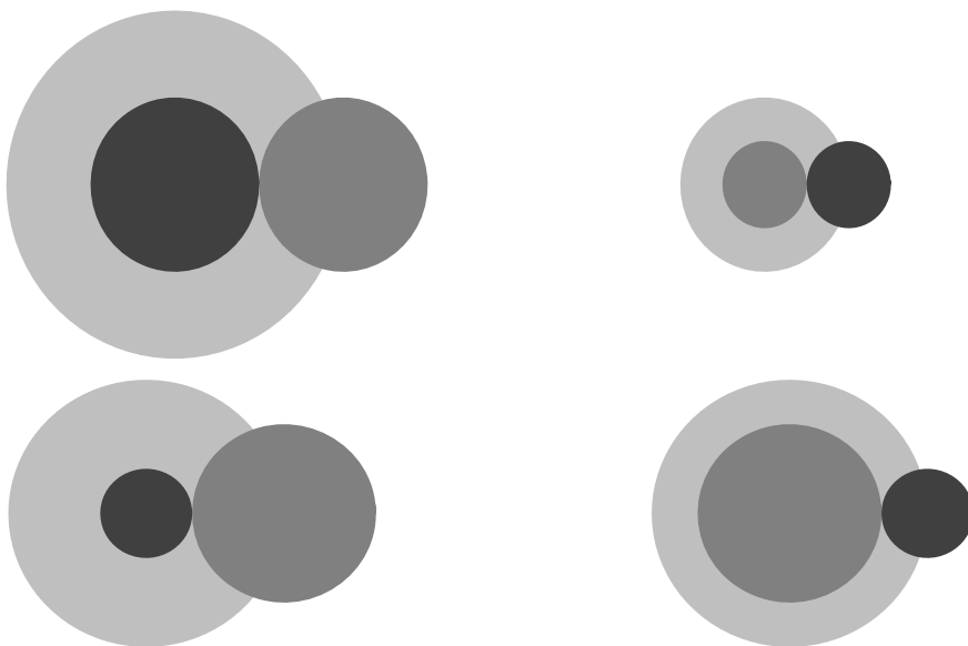
Fig. G.1 (a)–(b) Hard-core sphere of exclusion for homogeneous pairs. In a mixed gas composed of molecules with radii r_1 and r_2 , the size of the sphere of exclusion depends on the nature of the neighboring pairs. For pairs of type 1 molecules, the sphere of exclusion has radius 2r_1 . Similarly, for pairs of type 2 molecules, the radius of the sphere of exclusion is 2r_2 . The shading for the molecules is either dark or grey. The excluded volume is shaded very light-grey. (c)–(d) Hard-core sphere of exclusion for heterogeneous pairs. In a mixed gas composed of molecules with radii r_1 and r_2 , the size of the sphere of exclusion depends on the nature of the neighboring pair. When the pair consists of different types of molecules, the excluded volume is a sphere of radius r_1 + r_2 . Such a sphere—shaded very light-grey—can equivalently be considered to reside on either of the two molecules
