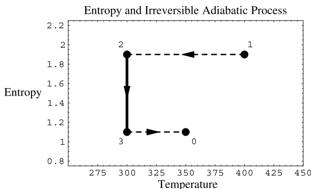
Fig. 4.4 Entropy/(J K -1 ) versus temperature/K. The scale shown is arbitrary. Broken lines are reversible adiabats and the full line is a reversible thermostat. The irreversible adiabatic process, that takes the system from the equilibrium state 0 to 1, passes through nonequilibrium states that cannot be displayed in the above plot. Note that S_3 = S_0 and S_2 = S_1 . Also, T_3 = T_2
