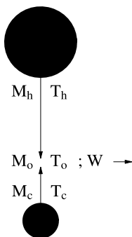
Fig. 4.7 Schematic plot for Problems 4.8 and 4.9. Two masses, m_h (specific heat C_h and at temperature T_h ) and m_c (specific heat C_c and at a lower temperature T_c ), are used as finite heat energy reservoirs for a perfect Carnot engine. When maximum work has been performed, the two masses reach a common temperature T_0 . Note that this temperature is lower than the T_f that is obtained when the two masses are put directly into thermal contact. (Compare with T_f shown in Fig. 4.6.) The heat energy content of the system at temperatures T_f and T_0 differs by W , the work output of a perfect Carnot engine. For convenience of display, m_h C_h and m_c C_c are represented as M_h and M_c , and their sum ( M_h + M_c ) as M_o
