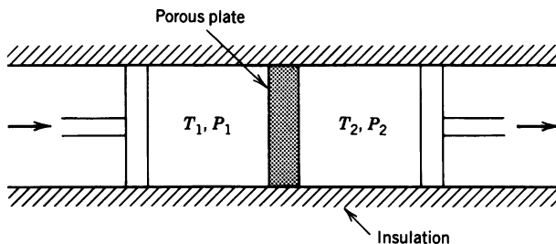
Fig. 7.2 Schematic view of the Joule–Kelvin apparatus
