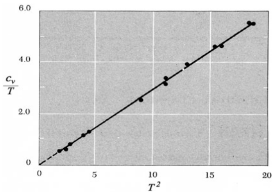
Fig. 11.19 As reported in [34], the plot presents the ratio \frac{c_v}{T} for KCl as a function of T^2 . Measurements are from Keesom, P.H., and Pearlman, N. Notice that there is no intercept. This indicates that at very low temperature, the specific heat varies as T^3 rather than as T . (The drawing is copied with permission from [35, Fig. 10.2.3])
