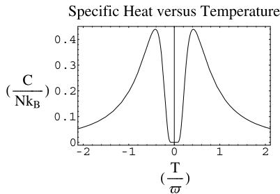
Fig. 11.17 The specific heat of the two-state nuclear paramagnet. At T = +0 the specific heat, as also shown in Fig. 11.10, is equal to zero—which is its minimum value. It rises—first slowly and then rapidly—with the increase in temperature and, as expected, undergoes a Schottky anomaly before trailing off toward its minimum value of zero as the temperature heads toward +\infty . Note that C(T) is symmetric with respect to the interchange of temperature, that is, C(+T) = C(-T)
