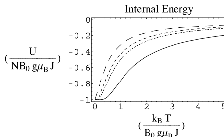
Fig. 11.9 Temperature dependence of the internal energy of the paramagnetic salt is plotted in dimensionless units. The solid curve refers to J = \frac{1}{2} , the thinnest, dashed curve is for J = \frac{3}{2} , the next higher curve refers to J = \frac{5}{2} , while the highest curve—with long dashes—represents the classical limit, i.e., J \rightarrow \infty
