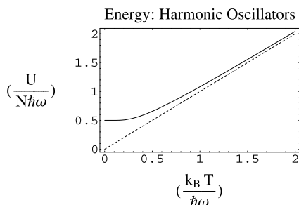
Fig. 11.4 Energy of a quantum and a classical simple harmonic oscillator. The solid curve represents the average energy of a quantum simple harmonic oscillator as a function of the dimensionless variable \gamma^{-1} = \frac{k_B T}{\hbar\omega} . The dashed curve represents the corresponding result for a classical simple harmonic oscillator
