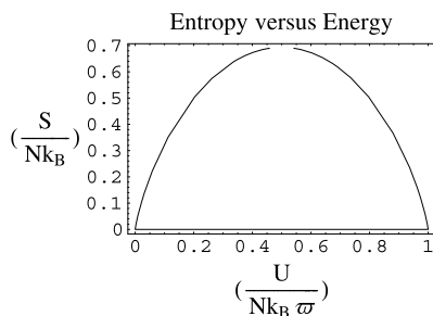
Fig. 11.16 Entropy S , in units of Nk_B , as a function of the energy U , in units of Nk_B\varpi , for a two state nuclear paramagnet. The shown value of the entropy is equal to zero at both the minimum value of the energy—i.e., at U = 0 —and the maximum value—i.e., at U = Nk_B\varpi . The entropy rises with the increase in temperature and seems to level off at its maximum value of Nk_B \ln(2(\frac{1}{2}) + 1) = Nk_B \ln(2) . Recall that S(T) is symmetric with respect to the temperature, that is, S(+T) = S(-T) . At the position marked by a small empty space in the otherwise continuous looking curve, the derivative (\frac{\partial S}{\partial U})_{V,N} changes its value from +0 to -0 , which indicates that at this point the temperature instantly changes from +\infty to -\infty . Note that the derivative (\frac{\partial(\frac{S}{Nk_B})}{\partial(\frac{U}{Nk_B\varpi})})_{N,V} is equal to \frac{\varpi}{T} —and its positivity from the position U = 0 to \frac{U}{Nk_B\varpi} = 0.5 indicates positive values of the temperature while its negativity in the range \frac{U}{Nk_B\varpi} = 0.5 \rightarrow 1 indicates negative values for the temperature. From left to right the temperature increases according to (T = 0 \rightarrow +\infty, -\infty \rightarrow -0)
