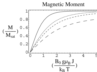
Fig. 11.8 The ratio \frac{M}{M_{\text{sat}}} is plotted as a function of \frac{B_0 g \mu_B J}{k_B T} . Here M represents the quasi-classical quantum statistical average of the system magnetic moment and M_{\text{sat}} its saturation value. The temperature is T and the magnetic field is B_0 . The solid curve refers to J = \frac{1}{2} ; the thinnest, dashed curve is for J = \frac{3}{2} ; the next lower curve refers to J = \frac{5}{2} ; while the lowest curve—with long dashes—represents the classical limit, i.e., J \rightarrow \infty . Notice that the solid curve has nearly reached its maximum possible value of unity when \frac{B_0 g \mu_B J}{k_B T} \approx 3 . For a J = \frac{1}{2} system, this means that the magnetic moment is close to reaching saturation when k_B T falls below B_0 \mu_B / 3 , or equivalently, when the ratio \frac{B_0}{T} rises above the value \frac{3k_B}{\mu_B} = \frac{3 \times 8.617343(15) \times 10^{-5}}{5.7883817555(79) \times 10^{-5}} (\text{eV K}^{-1} / \text{eV T}^{-1}) \approx 4.4662 \frac{\text{Tesla}}{\text{Kelvin}}
