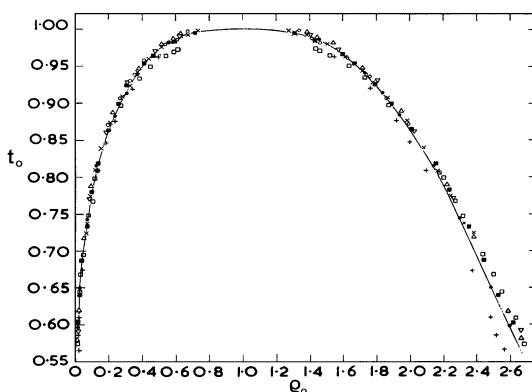
Fig. 6.7 Reduced Molar Densities in the Coexistent Regime. Experimental data—from [14]—for the reduced molar densities \rho_{0G} and \rho_{0L} —equal respectively to the inverse of the reduced molal volumes V_{0G} and V_{0L} —is displayed for a variety of fluids. Note, when \rho_0 < 1 , the displayed results are for \rho_{0G} . Similarly, the data for \rho_{0L} is displayed in the region where \rho_0 > 1 . The fluids studied are: argon, neon, krypton, xenon, nitrogen, oxygen, carbon monoxide, and methane. The ordinate is the reduced temperature t_0
