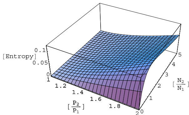
Fig. 5.2 For 1 \leq P_2/P_1 \leq 2 , and 0 \leq N_2/N_1 \leq 5 , twice the entropy increase/ [(N_1 + N_2)k_B] is plotted as a function of P_2/P_1 and N_2/N_1 . Despite its changed appearance, notice that the curve for N_2/N_1 = 1 is identical to that given in Fig. 5.1
