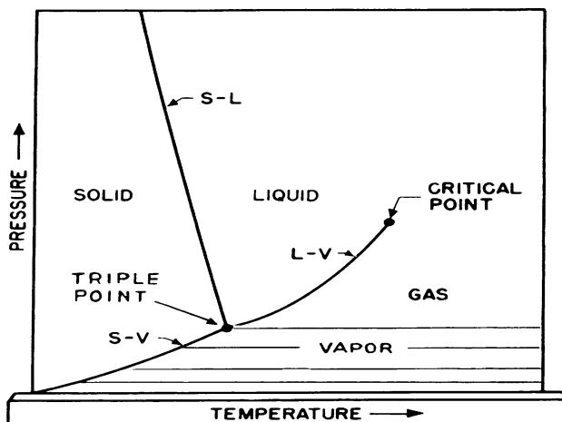
Fig. 10.2 Schematic plot of the Clausius–Clapeyron equations and the phase boundaries for \text{H}_2\text{O}
