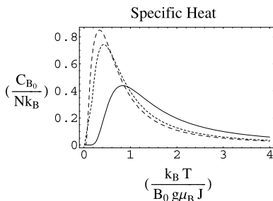
Fig. 11.10 Specific heat of paramagnetic salt at constant applied field, B_0 , is plotted as function of the temperature. The plot is in dimensionless units. The solid curve refers to J = \frac{1}{2} ; the short-dashed curve relates to J = \frac{3}{2} , while the curve with slightly longer dashes represents the case J = \frac{7}{2} . Notice that even though the difference in the J values is half as large, the separation between the bumps for J = \frac{3}{2} and J = \frac{1}{2} is noticeably greater than the corresponding separation between the bumps for J = \frac{7}{2} and J = \frac{3}{2} .
