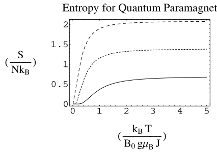
Fig. 11.7 Entropy of a quasiclassical quantum Langevin paramagnet as a function of \frac{1}{x} = \frac{k_B T}{B_0 g \mu_B J} . The solid curve refers to J = \frac{1}{2} ; the short-dashed curve relates to J = \frac{3}{2} , and the curve with slightly longer dashes is for J = \frac{7}{2} . Notice that at high end of the temperature scale, the curves are clearly heading toward their limiting value of \ln(2J + 1) . The plots are in dimensionless units
