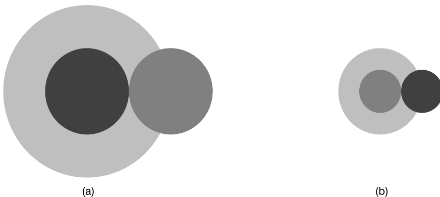
Fig. 6.1 Hard core sphere of exclusion for homogeneous pairs. For pairs of type 1 molecules—shown in (a)—the radius of the sphere of exclusion is 2r_1 . Similarly, for pairs of type 2 molecules—shown in (b)—the radius of the sphere of exclusion is 2r_2 . For simplicity the graph does not display the excluded volume for a nearest pair formed by one molecule of type 1 and another of type 2. In the description provided below, we initially treat only single type of molecules with radius of exclusion equal to 2r_0 . Later on, the case involving two different types of molecules is also considered. The shading for both types of molecules is dark and grey. The excluded volume is shaded very light-grey
