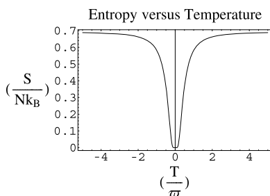
Fig. 11.15 Entropy S , in units of Nk_B , as a function of the temperature T , in units of w , for a two state nuclear paramagnet. Notice that the entropy is equal to zero—which is its minimum here—at T = +0 . It rises with the increase in temperature and, as the temperature heads to T \rightarrow +\infty , it seems to level off at its maximum value of Nk_B \ln\{2(\frac{1}{2}) + 1\} = Nk_B \ln\{2\} . Also notice that the entropy is symmetric with respect to the temperature, that is, S(+T) = S(-T)
