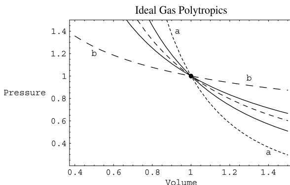
Fig. 3.2 Ideal Gas Polytropics. Plot for a monatomic ideal gas where \gamma = \frac{5}{3} . Curve a refers to \nu = 3 and curve b to \nu = 1/3 . In-between these curves, in seriatim lie curves for \nu = 5/3 , referring to the isentropic case and shown here as the full curve nearest to a ; \nu = 1.25 , dashed curve that lies between the two full curves; and \nu = 1 , referring to the isothermal case and shown as a full curve nearest to b . Note that specific heat cannot be defined for the cases represented by the full curves. Also note that the polytropic specific heat would be negative for all cases represented by curves that lie in-between the two full curves. On the other hand, for all those polytropic processes that can be represented by curves that lie outside the two full curves, the polytropic specific heat would be positive
