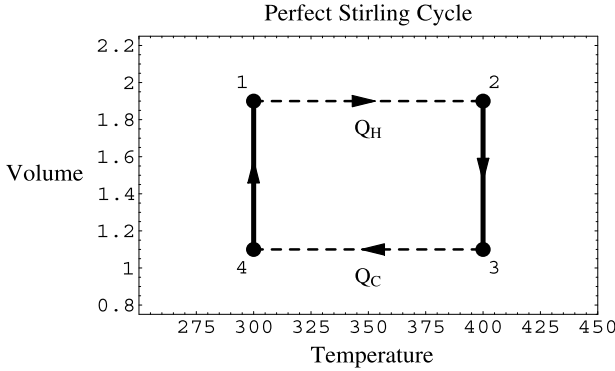
Fig. 4.9 Temperature versus volume. Here Q_H = Q^{\text{rev}}(T_H) and Q_C = Q^{\text{rev}}(T_C) . Full lines are thermostats and broken lines isochors. Scale is arbitrary
