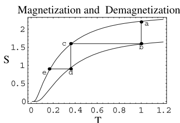
Fig. 11.11 Shown above are instances of a paramagnetic crystal under isothermal increase in the applied field followed by reversible adiabatic decrease of the same. This is a schematic plot and arbitrary scale is used for both the entropy S and the temperature T . While the upper curve refers to the system being under a weak applied field, the magnetic field for the lower curve is relatively strong. The journey from point a to b represents isothermal magnetization of the paramagnetic salt. Here heat energy is released by the salt to the helium reservoir. During the final part of the journey, which takes the system from b to c , the magnetic field is reduced back to its original strength. This travel occurs reversibly and adiabatically. Hence it is isentropic. A consequence of (11.180) and (11.175) is that in any of the given processes, when the entropy, S , is constant, the magnetization, M , is also constant. Therefore, during the travel from b to c , the system magnetization also remains constant. Accordingly, in addition to being isentropic, this process is also “isomagnetic.” Clearly, calling it “adiabatic demagnetization” is a misnomer! More importantly, the process from b to c lowers the system temperature from that of the liquid helium reservoir—recall that both points a and b are at the same temperature that is set by contact with the liquid helium reservoir—to that of point c . If another reservoir at the lower temperature represented by the point c were also available, then a similar two-step process could be repeated. In this fashion, the system would move from c to a point shown as d and then onto a point e at an even lower temperature
