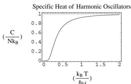
Fig. 11.5 Specific heat of a quantum and a classical simple harmonic oscillator. The solid curve represents \frac{C}{Nk_B} of a quantum simple harmonic oscillator as a function of the dimensionless variable \gamma^{-1} = \frac{k_B T}{\hbar\omega} . The dashed curve represents the corresponding result for a classical simple harmonic oscillator. Remember C_p = C_v = C
