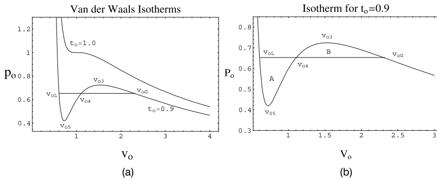
Fig. 6.2 (a) (p_0, v_0) -plot of the Van der Waals isotherms for t_0 = 1.0 and 0.9 . (b) (p_0, v_0) -plot of the Van der Waals isotherm for t_0 = 0.9
