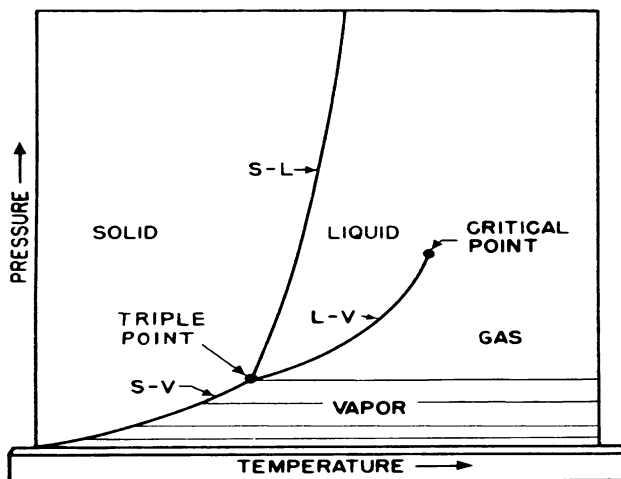
Fig. 10.1 Schematic plot of the Clausius–Clapeyron equations and the phase boundaries for real substances except \text{H}_2\text{O}
