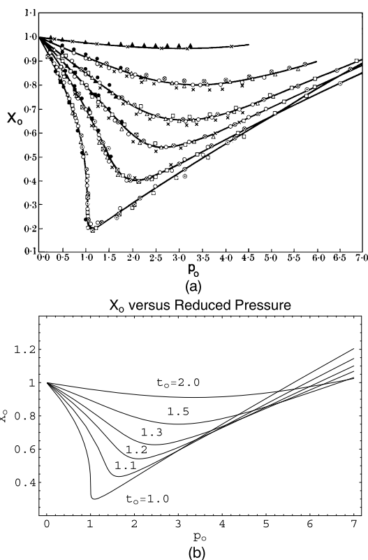
Fig. 6.5 (a) Experimental Results for X_0 as function of p_0 . For a variety of fluids, X_0 is plotted as a function of the reduced pressure. The fluids represented are: carbon dioxide, ethane, ethylene, isopentane, methane, n -butane, n -heptane, nitrogen, and water. The experimental results are qualitatively similar to those predicted by the Van der Waals theory. Data fit remarkably well onto curves that are almost identical for different fluids. To avoid cluttering up the figure, the curves have not been labeled. Top curve refers to t_0 = 2.0 . In descending order, t_0 for the next four lower curves is = 1.5, 1.3, 1.2, 1.1, 1.0 . (Data from [11].) (b) X_0 versus p_0 . Van der Waals theory results for X_0 versus p_0 . The curves follow almost the same pattern as the experimental results shown in panel a
