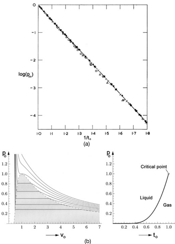
Fig. 6.8 (a) Reduced vapor pressure in the coexistent regime. The fluids studied are: argon, krypton, xenon, nitrogen, oxygen, carbon monoxide, and methane. Note that the curve appears to be a straight line, indicating a linear drop with 1/t_0 , which is equivalent to a functional dependence of the form p_{00} \propto t_0^\nu with \nu \sim 7.3 . (b) Reduced vapor pressure in the coexistent regime for a Van der Waals gas. The figure on the left-hand side shows Maxwell isobars on a P - V plot. Each such isobar has a corresponding temperature which is not shown in this figure. The figure on the right-hand side displays the pressure of such isobars against their corresponding temperature, both on the reduced scale. (This plot is reproduced courtesy of [16])
