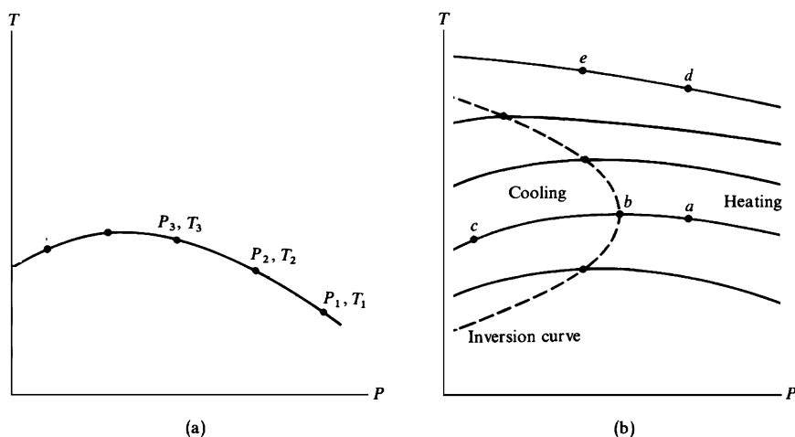
Fig. 7.3 Schematic view of the Joule–Kelvin experiment results. Each smooth curve refers to a constant value of the entropy while the dotted curve (b) represents the locus of the inversion points
