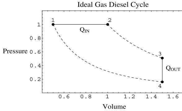
Fig. 4.10 Diesel cycle using ideal gas as the working substance
