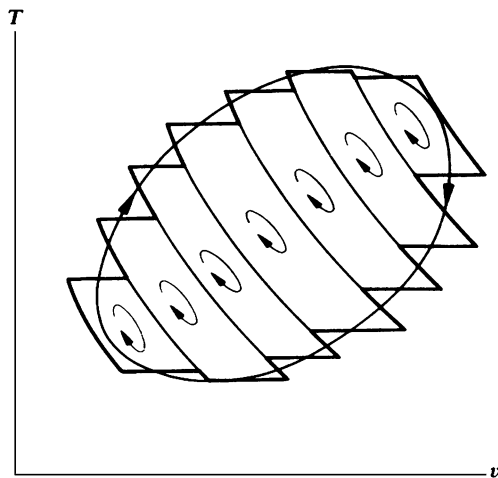
Fig. 4.2 Any arbitrary shaped, finitely sized, reversible cycle can be approximated by a very large number of extremely tiny Carnot cycles. In the figure above, the adiabats in successive contiguous tiny Carnot cycles are seen approximately to cancel each other out—that is, adiabat IV from cycle i cancels the adiabat II in cycle i + 1 . Note that such cancelation becomes perfect—meaning, exact—when the cycles are infinitesimally small. Furthermore, the jagged structure of the uncanceled parts smoothes out to the desired arbitrary shaped, finitely sized, reversible cycle. (This sketch is similar to that given in [1])
