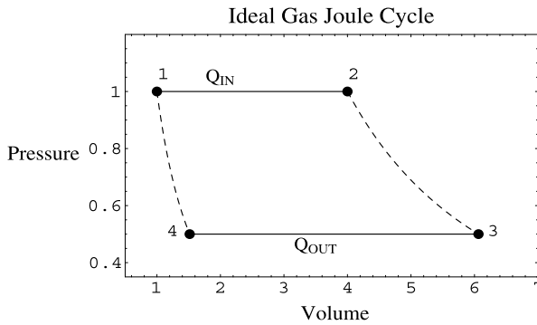
Fig. 4.12 Joule cycle using ideal gas as the working substance
