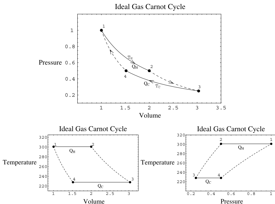
Fig. 4.1 (a) Pressure/( 5 \times 10^5 ) Pa versus volume/( 10^{-2} m 3 ). Here Q_H = Q^{\text{rev}}(T_H) and Q_C = Q^{\text{rev}}(T_C) . Full lines are isotherms and broken lines adiabats. (b) Temperature/(K) versus volume/( 10^{-2} m 3 ). Here Q_H = Q^{\text{rev}}(T_H) and Q_C = Q^{\text{rev}}(T_C) . Full lines are isotherms and broken lines adiabats. (c) Temperature/(K) versus pressure/( 5 \times 10^5 ) Pa. Here Q_H = Q^{\text{rev}}(T_H) and Q_C = Q^{\text{rev}}(T_C) . Full lines are isotherms and broken lines adiabats
